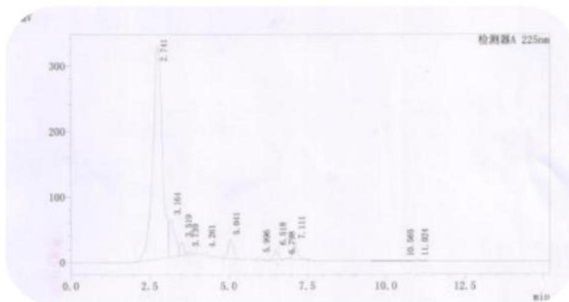
Our chromatogram
